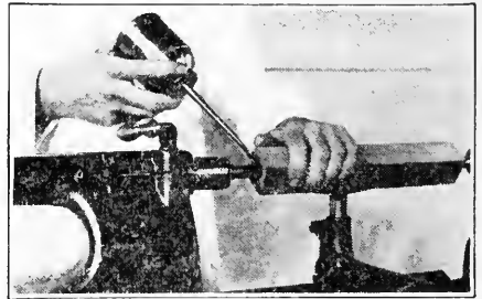
FIG. 286. OILING DEAD CENTER.
